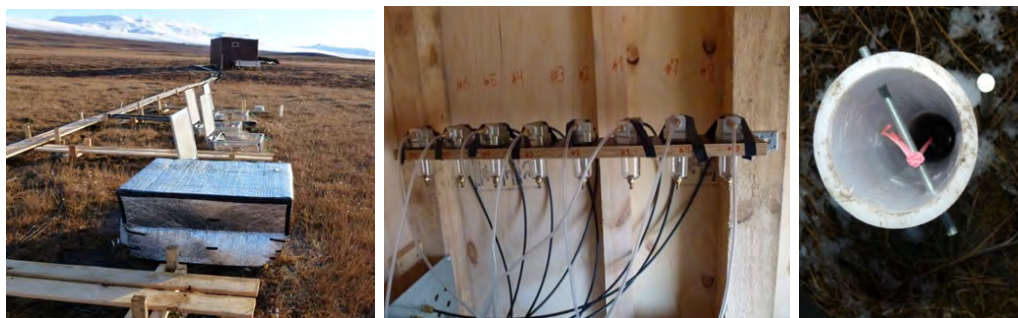
Figure 80: Chamber 2 covered with box for dark chamber measurements (left). Water traps inside the hut (mid). Looking into white tube with diver (right).
