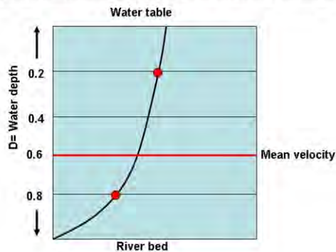
Figure 51: Standard velocity profile in the river and an example of measuring velocity at two different water depths.
