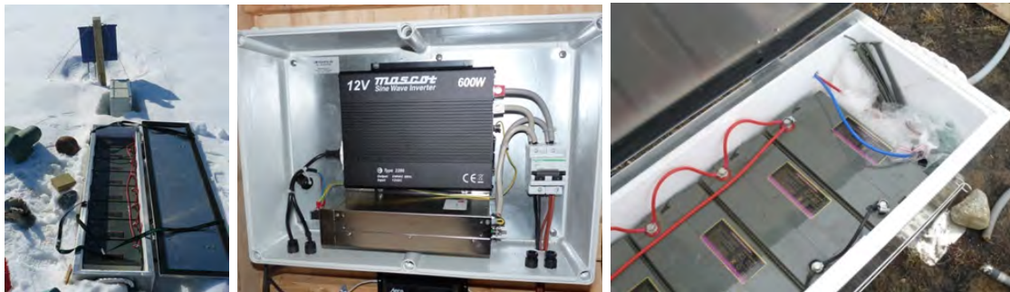
Figure 77: The battery box (left). A look into the transformer box, inside the hut (mid). Power cable from the instrument box enters the battery box in the southern end –the red and blue cable are connected to plus and minus on the last battery in the row.
