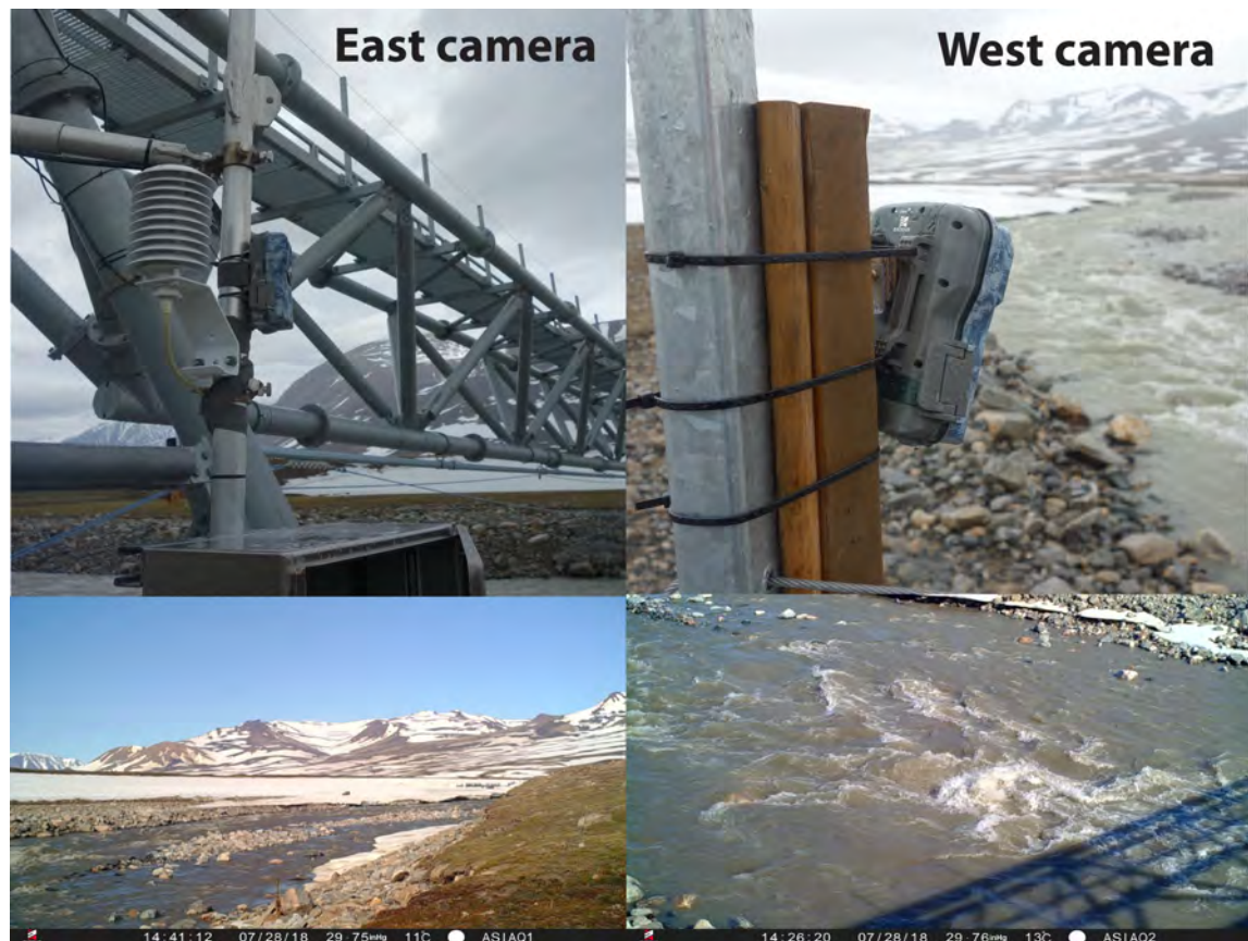
Figure 46: Camera mountings and frames for the time lapse cameras on the bridge.
