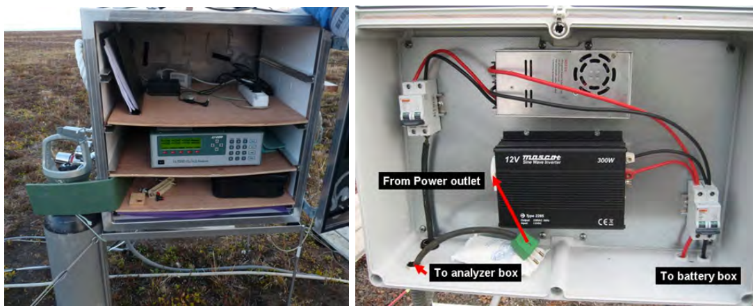
Figure 71: A look inside the enclosure, with the Licor7000, connected the eddy mast and the Nitrogen gas (on the left side of the enclosure) (left). A look inside the transformer box (right).
