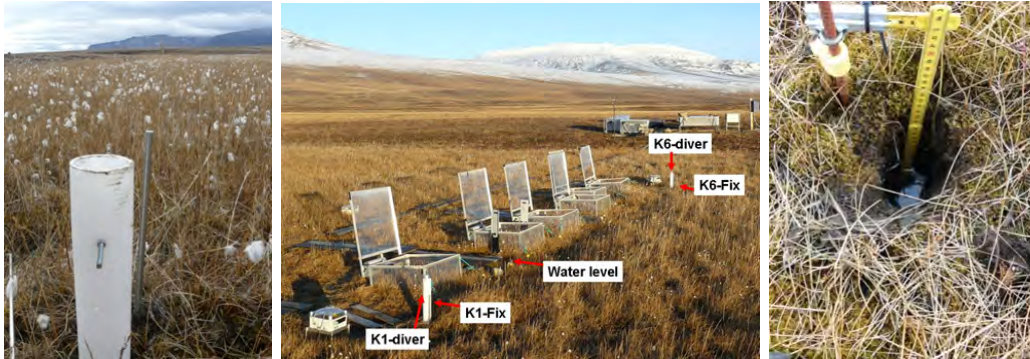
Figure 79: The diver tube K6-diver and the metal probe K6-Fix. The diver is placed so it hangs in a string from the screw that crosses the tube near the top (left). Overview of the methane site with divers and water level site (mid). The water level site (WLS) (right).
