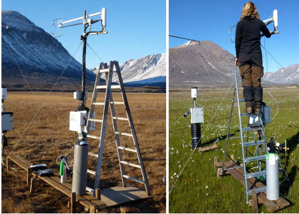
Figure 76: Setup for span testing or calibrating Licor7200. Left; the ladder is used for connecting or disconnecting the Bev-a-line tube for the air intake on the mast (where the white tube is connected to the licor house), Nitrogen and span gas, the computer is connected to the Licor7200 underneath the white enclosure using a RS232 cable. Right; calibration ‘in action’ the reference gas is connected to the licor7200 through the bev-a-line tube and in situ measurements are read from the PDA and noted in the calibration sheet.
