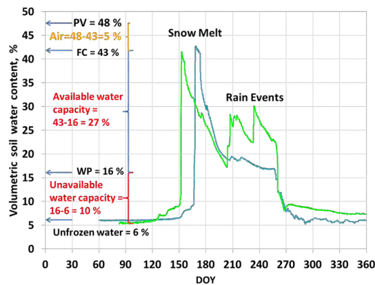
Figure 63: Volumetric soil water content for a sandy soil in a wet summer (light green) and a dry summer (blue). The Pore Volume (PV) is 48 %, the Field Capacity (FC) is 43 % (at the start of the thawing season) and Wilting Point (WP) is approximately 16 %. The Plant Available Water Capacity changes during the summer season with a steady drop in the dry summer and a drop with several rapid increases during rain events in the wet summer. Of the 16 % Unavailable Water Capacity 10 % changes phase between water and ice during thawing in the spring and freezing in the autumn, while 6 % remains unfrozen during the winter season.
