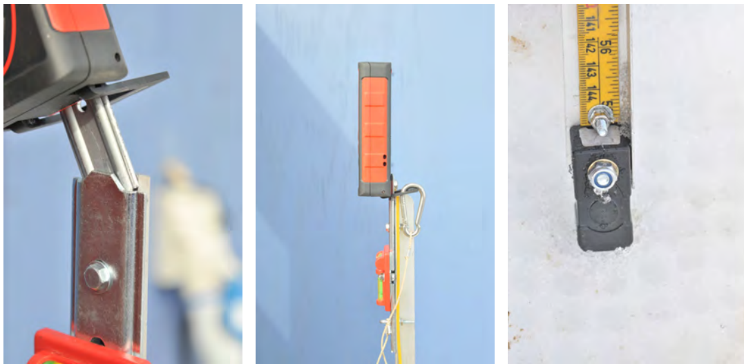
Figure 47: Correct mounting of range finder on pole with ruler (two leftmost photos) and placement of pole foot on a point directly under the hoist trolley (right photo).
