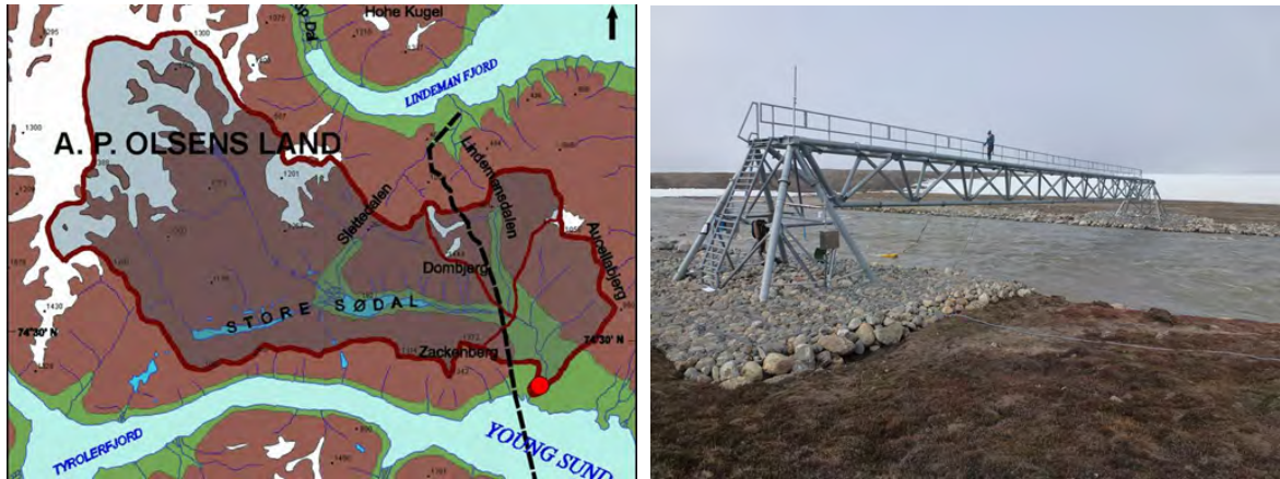
Figure 43: Map showing the Zackenberg drainage basin ( 512 \text{ km}^2 ). The hydrometric station (red dot) is located approximately 1-2 km up streams from where the Zackenberg River drains out in Young Sound (left). A photo showing the bridge and surroundings of the hydrometric station.
