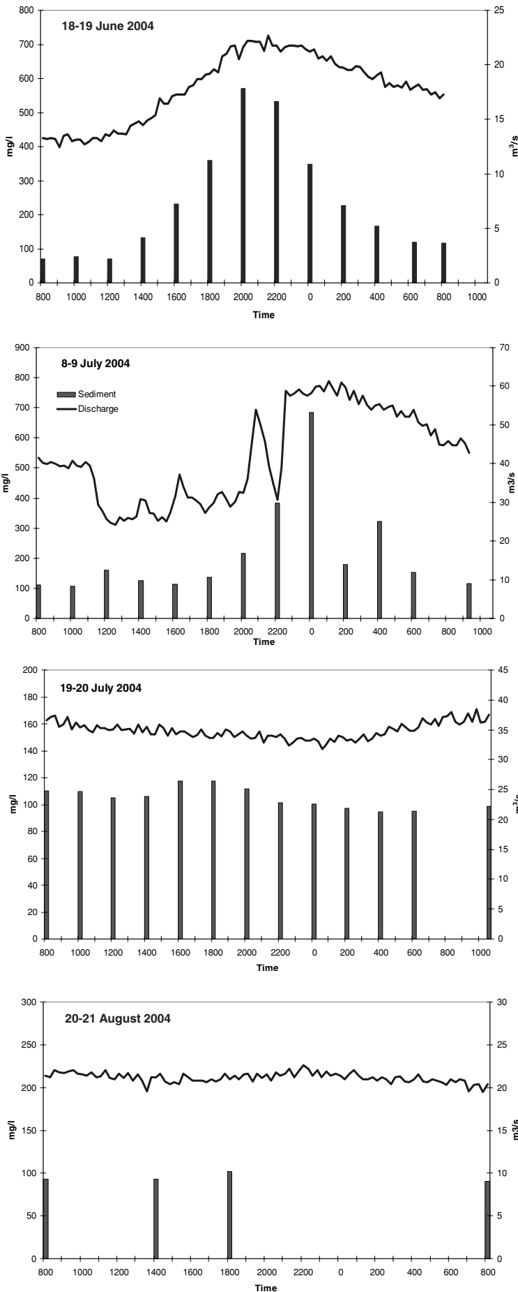
Figure 2.15. Corresponding sediment concentration (mg/l, shown as bars) and water discharge (m 3 /s, shown as line) in Zackenbergelven during four diurnal measurements throughout the season. From top: 18-19 June, 8-9 July, 19-20 July, 20-21 August. The variation in patterns reflect different weather situations and different parts of the season (see text). Notice different values on Y- axes.
