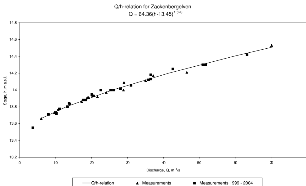
Figure 2.12. Water level – discharge relation curve (Q/h-relation) for Zackenbergelven at the hydrometric station, 1995-1998. The coefficient of correlation ( R^2 ) for the curve is 0.99. Measurements from the period 1999-2004 indicate that no major changes have occurred to the river profile since 1998.
