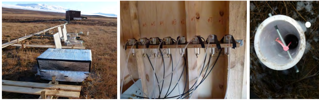
Figure 79: Chamber 2 covered with box for dark chamber measurements (left). Water traps inside the hut (mid). Looking into white tube with diver (right).
