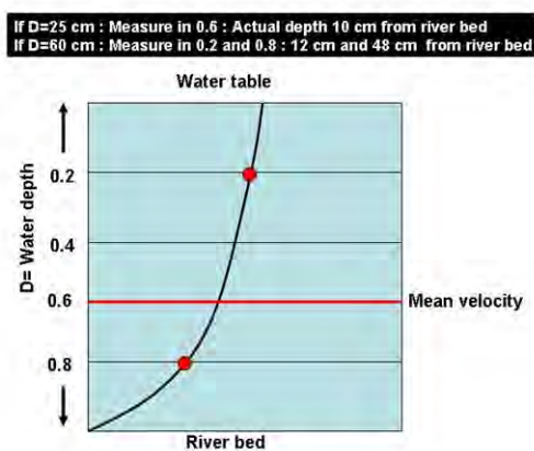
Figure 50: Standard velocity profile in the river and an example of measuring velocity at two different water depths.
