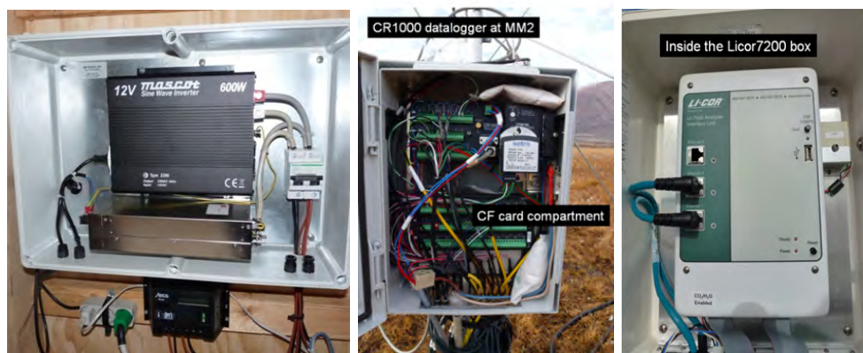
Figure 73: Left: Inverter inside the hut at MM2. Middle: look inside the CR1000 data logger box. Right: look into the Licor7200 box.
