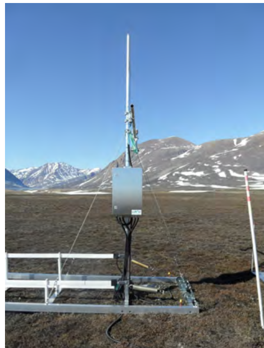
Figure 13: Snow Pack Analyzer. Looking West towards Zackenberg Mountain.
