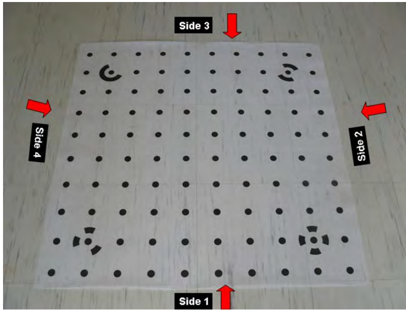
Figure 27: Calibration chart on the floor in House 1.
