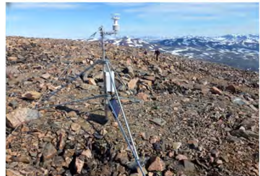
Figure 7: Meteorological station M8 close to the top of Zackenberg. Looking West towards the Aucella slope.
