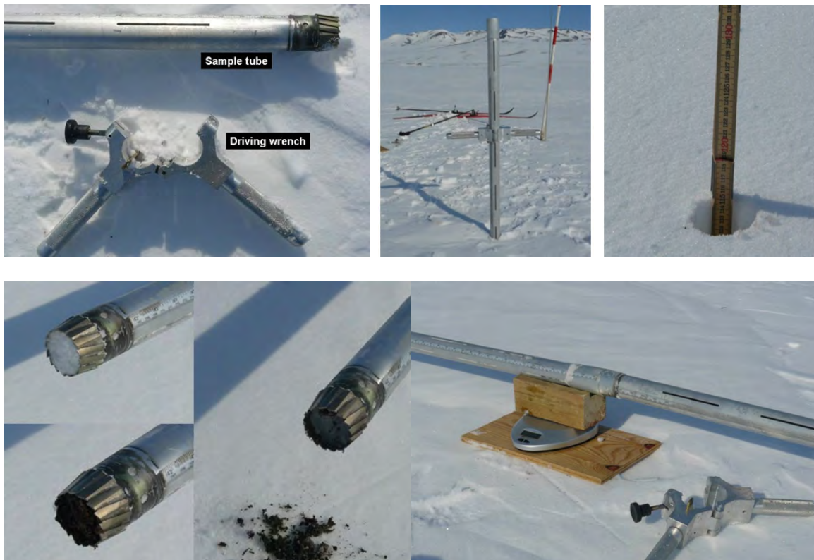
Figure 20: Snow sampling tube in use.
