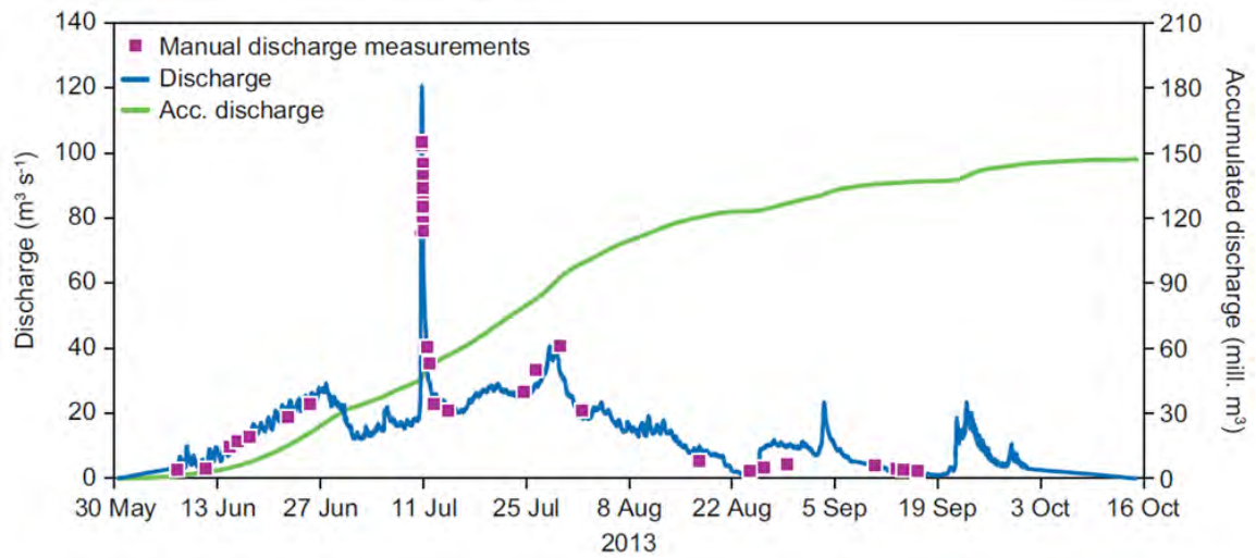
Figure 42: A typical season's discharge of Zackenberg river with manual discharge measurements (purple squares), the derived discharge time series (blue) and the accumulated discharge (green line).
