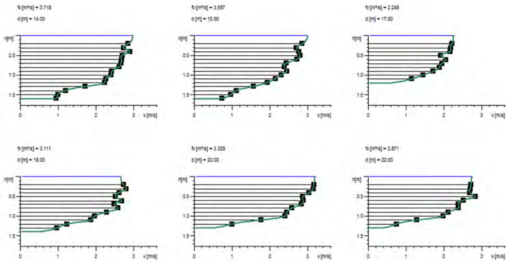
Figure 40: Example of flow velocity profiles at Zackenberg river on 16.08.2014. Note, that not all profiles follow a perfect logarithmic curve.
