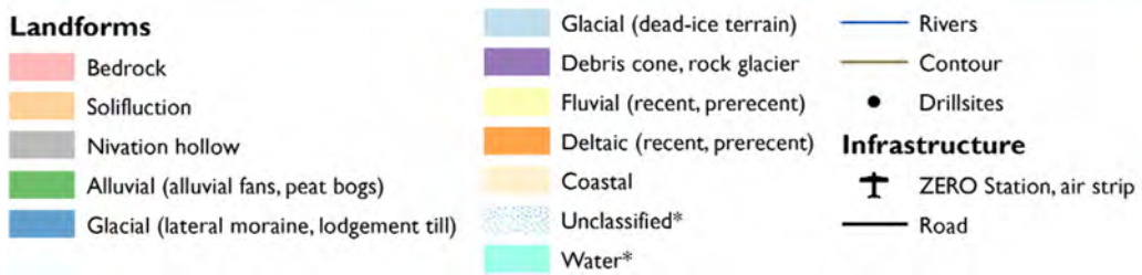
Figure 2: Geomorphological map of the Zackenberg valley (Cable et al., 2017)
