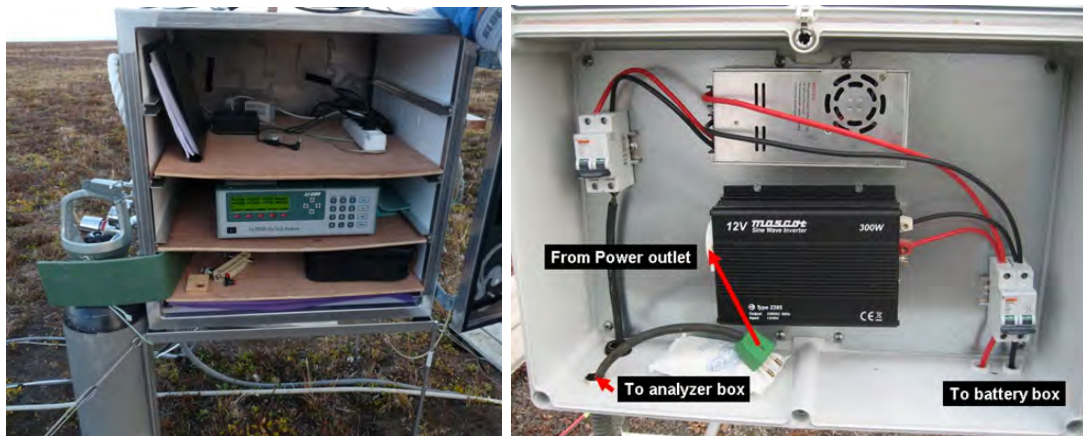
Figure 70: A look inside the enclosure, with the Licor7000, connected the eddy mast and the Nitrogen gas (on the left side of the enclosure) (left). A look inside the transformer box (right).
