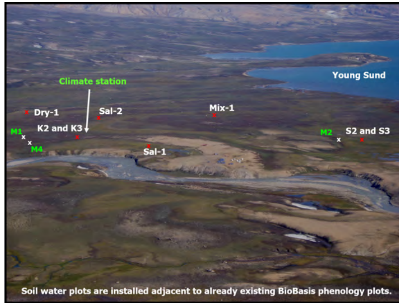
Figure 63: Photo looking Southeast from Nansen blokken. Location of soil water plots are marked by red crosses. Meteorological stations are marked by white crosses. Zackenberg station and the runway are in the center of the photo.
