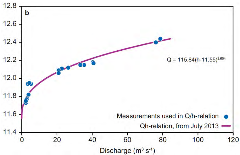
Figure 41: The Q/h relation for Zackenberg river for late 2013 with manual measurements (blue dots) and the derived relation (purple line). A new one had to be established after the GLOF from July 2013.
